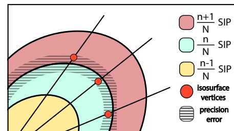
Figure 13: Illustration of the magnitude of SIP isosurface error with spherical sampling. For a SIP isosurface of iso-value \frac{n}{N} , the SIP isosurface error is on the scale of precision error. In our experiments, the error is less than 1e^{-12} . The SIP value of a point evaluates to \frac{n}{N} (blue) or \frac{n+1}{N} (red) depending on the precision error. The SIP isosurface vertices are red. The shaded area marks the precision error.
